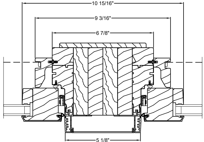
2 3/4" Solid Spread Mull
