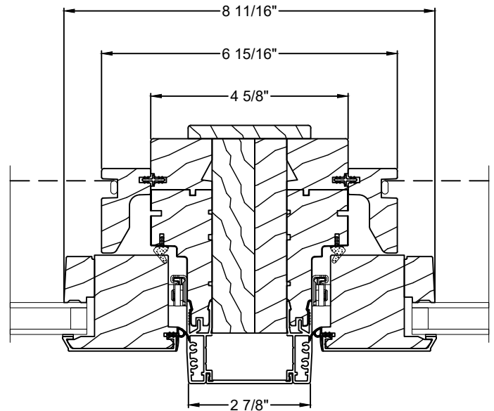
1 3/4" Solid Spread Mull
