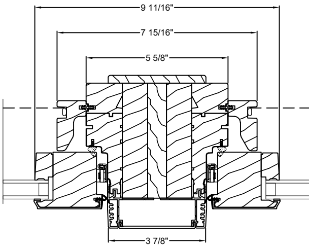
4" Solid Spread Mull
