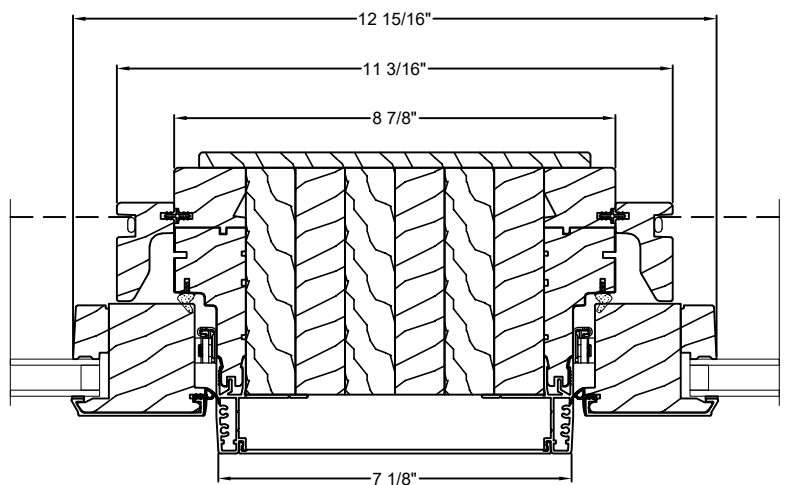
6" Solid Spread Mull
