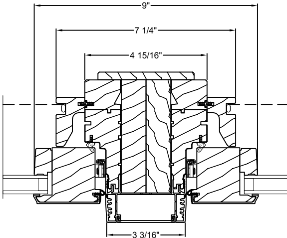
2" Solid Spread Mull
